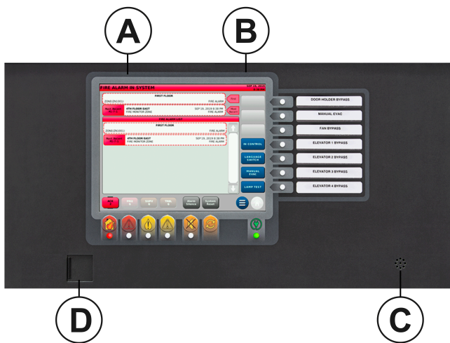
Figure 3: ES Touch Screen Display interface
