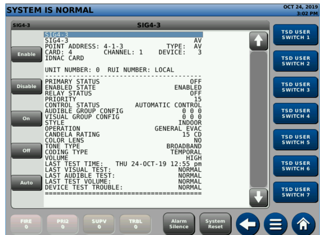
Figure 15: Detailed point status screen for TrueAlert ES appliance
