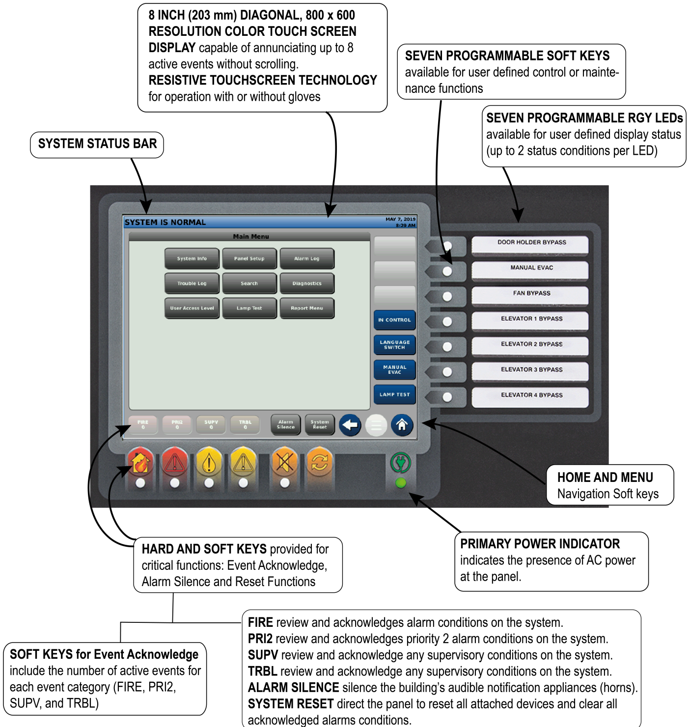
Figure 9: ES Touch Screen Display operator interface
