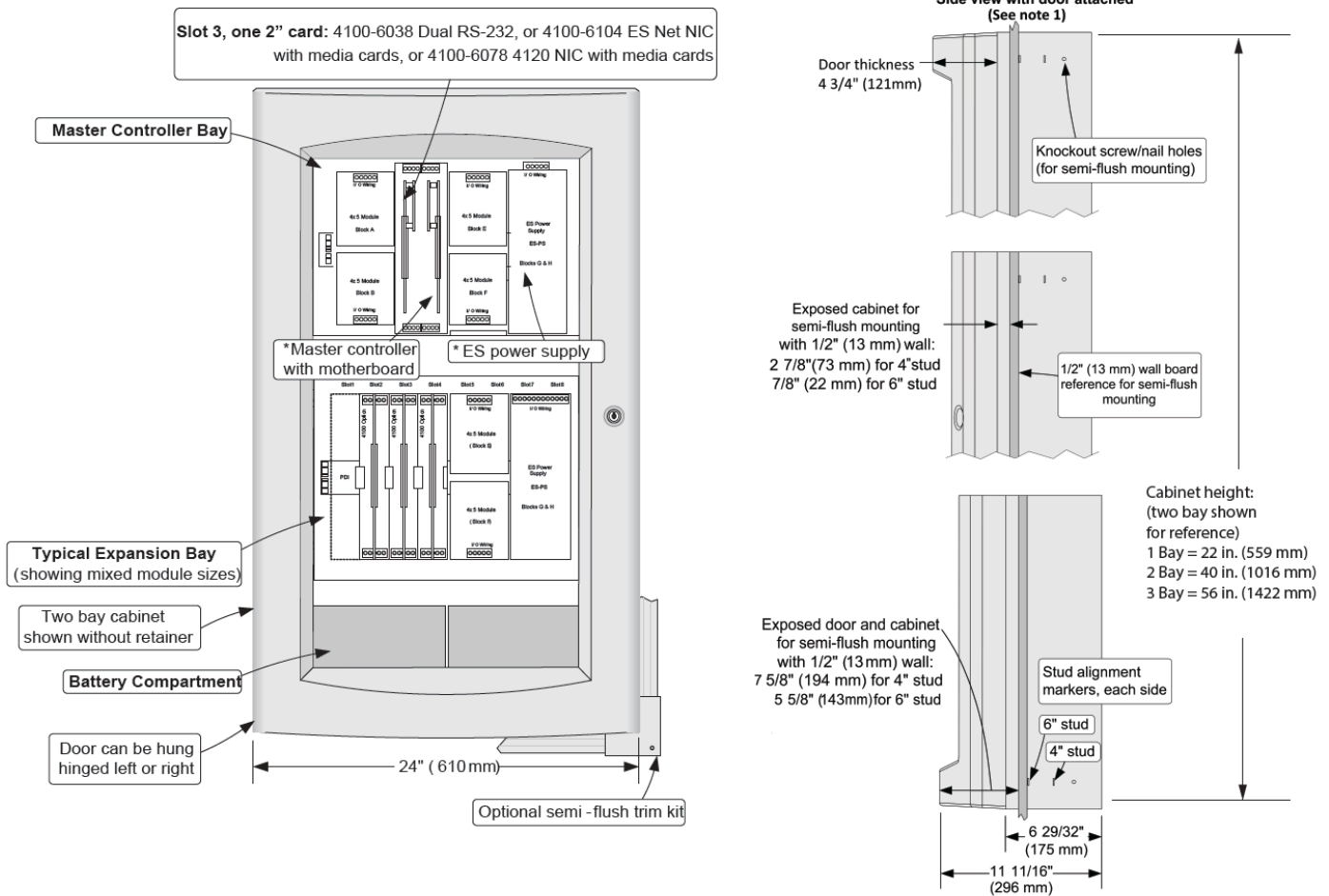
Figure 18: Mounting and CPU Bay module reference
